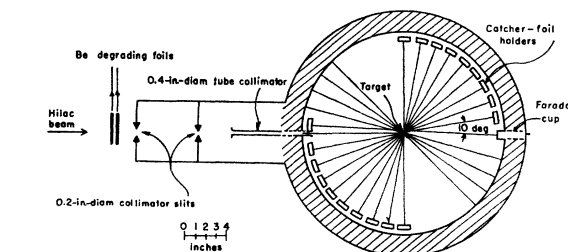
FIG. 1. Diagram of angular-distribution chamber.
