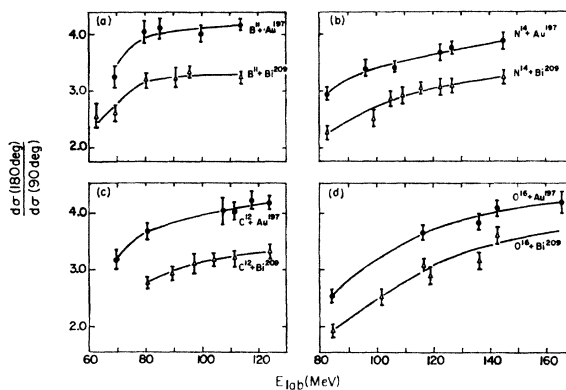
FIG. 5. Variation of the center-of-mass anisotropy with bombarding energy for (a) \text{B}^{11} , (b) \text{N}^{14} , (c) \text{C}^{12} , and (d) \text{O}^{16} incident upon both \text{Au}^{197} and \text{Bi}^{209} targets.
